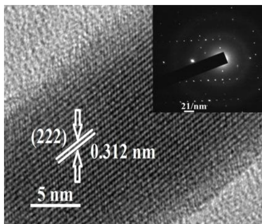
Figure: Lattice fringe pattern of the unknown nanorod system
